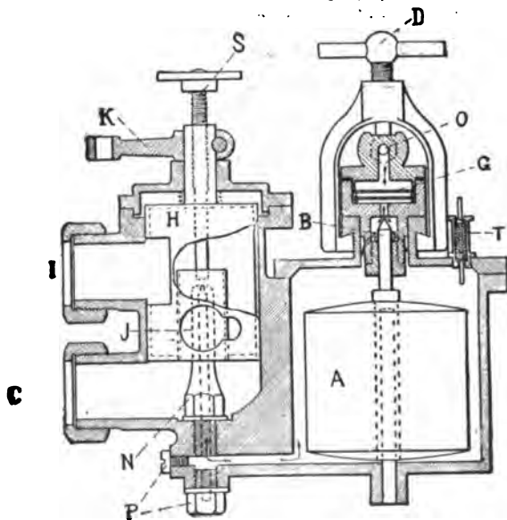
FIG. 282.—Section through a typical Float-Feed Carburetter. This particular device is the one shown in the previous cut. Here A is the hollow cylindrical float; B, the spindle of the needle valve; C, tube for admitting hot air around base of spraying nozzle; D, adjusting screw for the needle valve; H, adjustable air valve; I, outlet for fuel mixture to cylinder; J, adjustable opening for air; K, arm for attaching throttling lever; N, spraying nozzle; O, P, screw caps on channel from float chamber; S, adjusting screw for regulating gasoline spray; T, air vent; G, filtering gauze.
